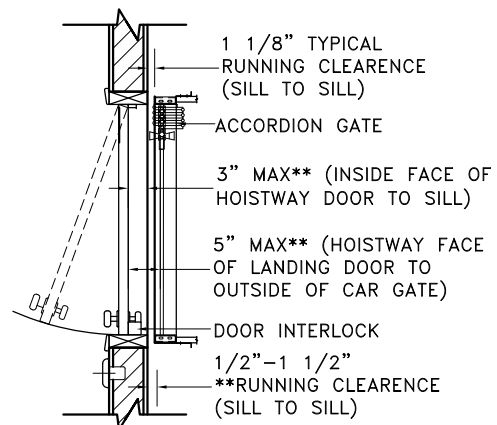
TYPICAL DOOR LOCATION DETAIL
